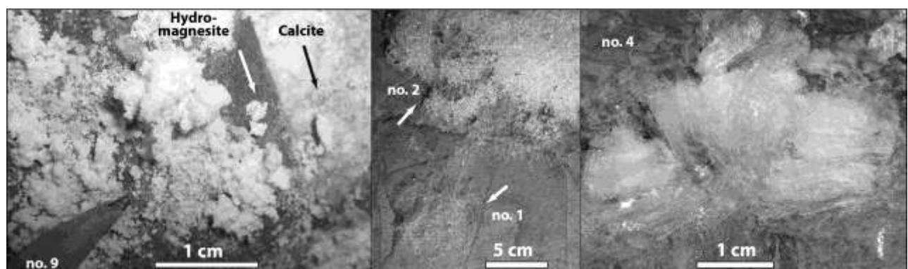
Fig. 2: Left picture: calcite spot occurring as wall coating originating from small percolation along a fissure, ringed by hydromagnesite cotton-like bundles [sample no. 9]. Central and right pictures: diverse mirabilite crystal fabrics. Candy floss-like filaments [sample no. 1]; melting snow-like isometric crystals [sample no. 2]; ice clear blades forming a flower [sample no. 4].
