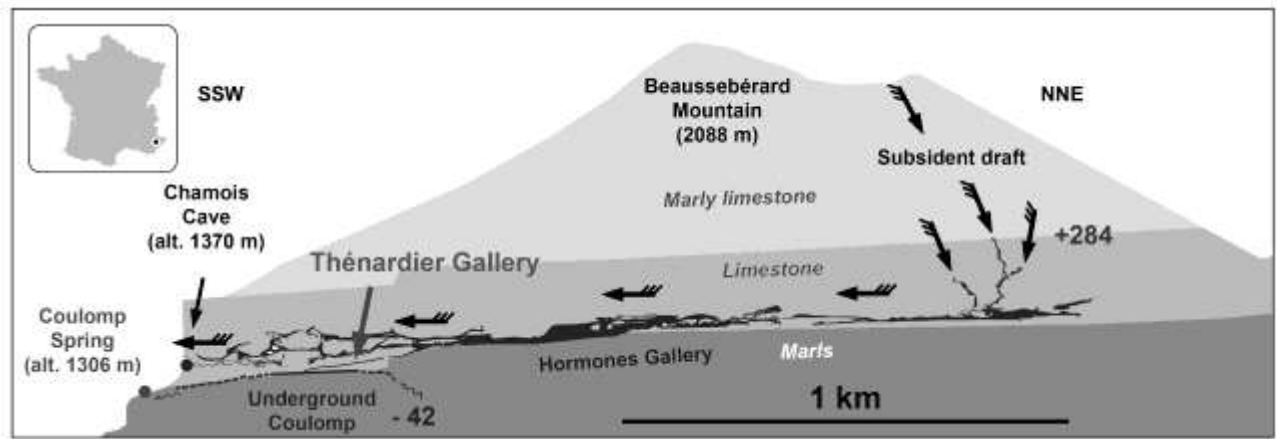
Fig. 1: Cross section of the Chamois Cave, showing its development below a narrow ridge, at the contact of a marly basement and in a limestone covered with a thick sequence or marly limestones. Strong draft entering at high altitude crosses the cave system towards the cave entrance. The Thénardier gallery is a tributary of the river, the Underground Coulomp, which is most of the time confined between sumps.
