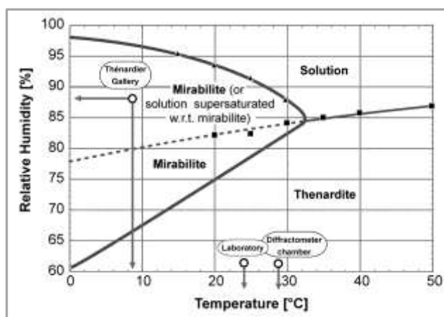
Fig. 5: Phase diagram for sodium sulfates. The continuous lines indicate the boundaries of the stable phases. Triangles and squares are experimental data for mirabilite and thenardite, respectively. The discontinuous line corresponds to a solution in metastable equilibrium with respect to thenardite and supersaturated with respect to mirabilite [figure extracted from FLATT, 2002 experiments, redrawn]. Note that the phase diagram of HILL & FORTI (1997, p. 192) displays the mirabilite-thenardite boundary line, constructed from one field case, in a slightly lower position (i.e. with drier conditions). We plotted the T - RH conditions of the Chamois Cave and of the Laboratory where X-ray analyses have been done, which clearly show that they are in the stability field of mirabilite and thenardite, respectively.
