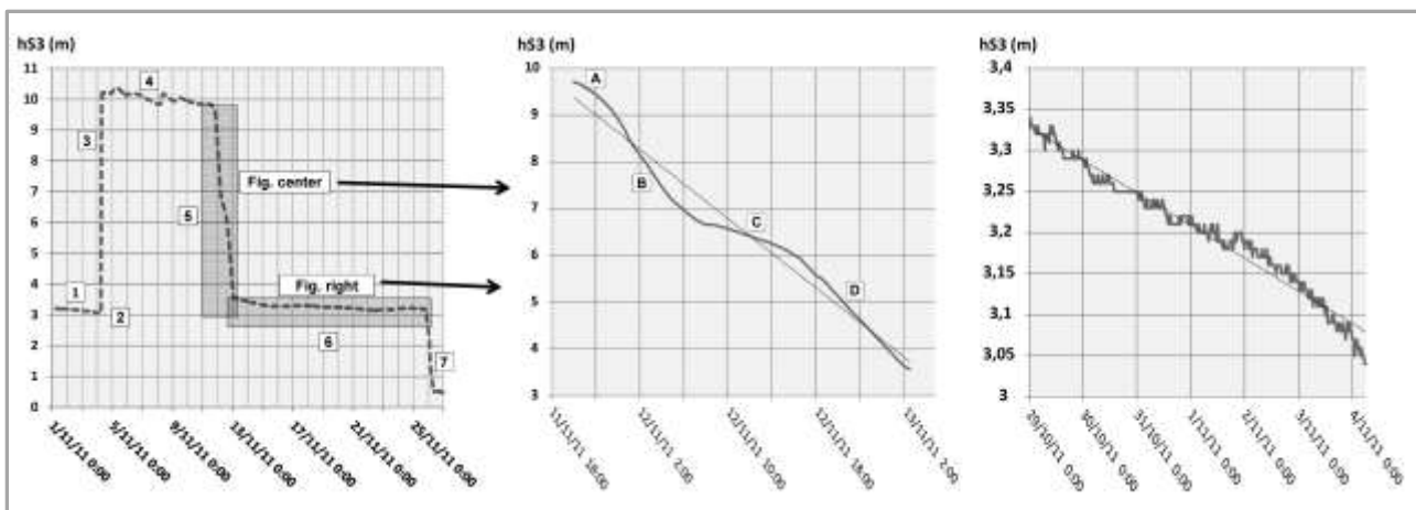
Fig.4: Flooding record in the S3 of Chamois Cave. (1) Low stable level of the sump, with very slow depletion from the last flood; (2): Rain starts on 3 Nov. 09:00 in Méailles, the flood in S3 begins on 4 Nov. 06:10; (3) S3 fills up over 7 m in 55 min. and pours out in Shadoks Gallery; (4) S3 remains active during 1 week till 11 nov., rains having stopped 60 h before; (5) fast depletion in 34 h of S3 level down to its low stable level (detail on central figure; letters correspond to the inclination changes of the emptying passage, see fig. 5); (6) very slow depletion similar to (1). Small peaks are electronic device artifacts (detail on right figure); (7) pumping of the S3 to reopen the access to the cave.
