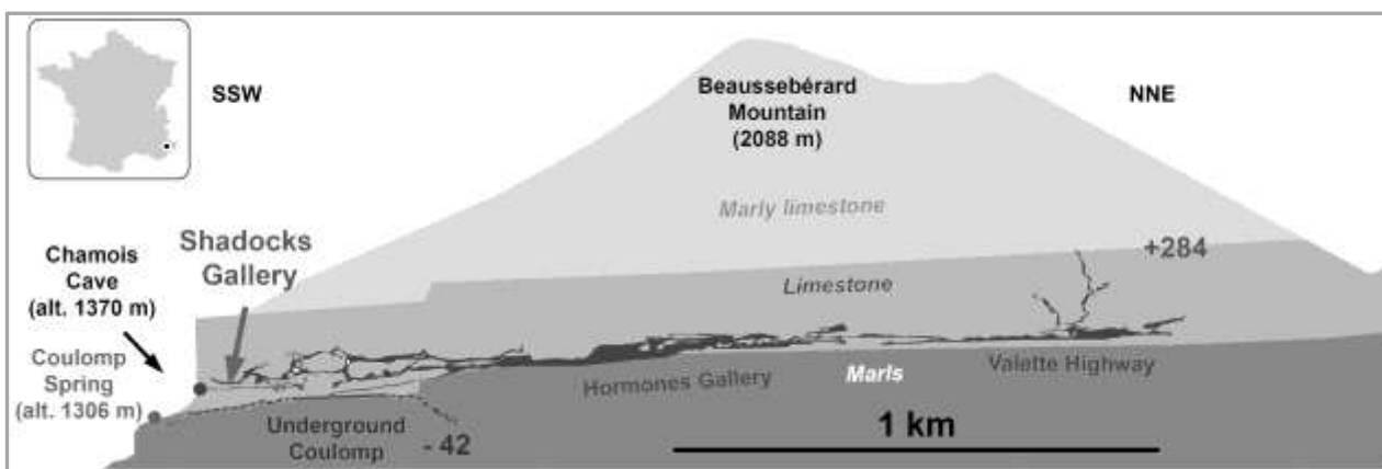
Fig. 1: Cross section of the Chamois Cave, showing its development at the contact of a marly basement and in a limestone covered with a thick sequence of marly limestones. In summer, strong draft entering at high altitude crosses the cave systems toward the entrance, as a simple wind tube.
