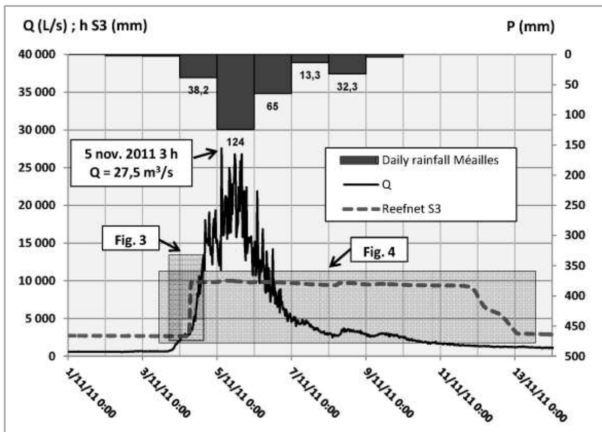
Fig. 2: Flood event of Nov. 2011 showing rainfall at the Méailles station, the Coulomp spring discharge, and the level on 3 rd sump (S3) in Chamois Cave. The fluctuations correspond either to real discharge pulses or to turbulences in the pool.
