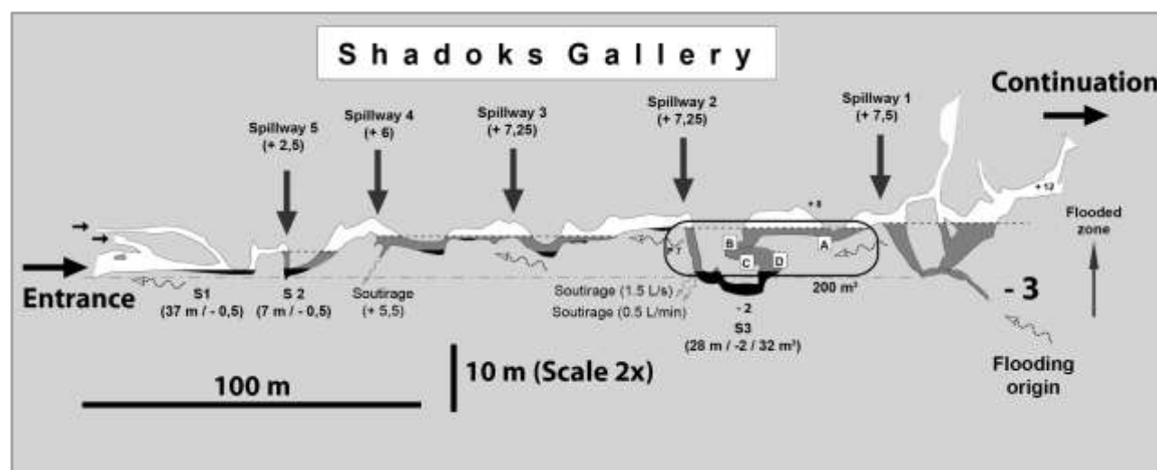
Fig. 5: Flooding of the Shadoks Gallery. Water rises from the right, and fills the S3 sump. During large floods, water rises in the S3, pours over spillway 2, and successively pours over the 3 next spillways. Volume flooded in S3 is about 200 \text{ m}^3 ; letters [A], [B], [C], [D] correspond to the first stage of fast emptying of S3 (see fig. 4 center and text).
